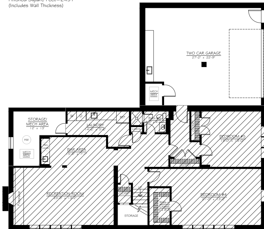
LOWER LEVEL Finished Square Feet = 1570 (Includes Wall Thickness)
